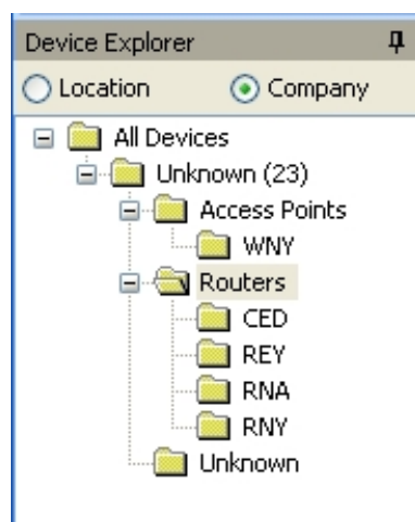
Fig. 4: Device Explorer
