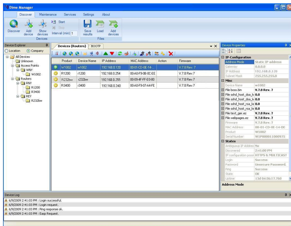
Fig. 2: Dime Manager
