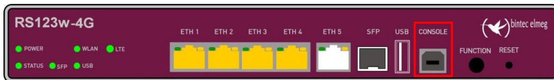
Fig. 15: CONSOLE Connector
