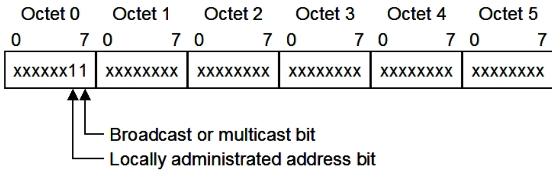
Fig. 2: IEEE 802.3 MAC address format.
