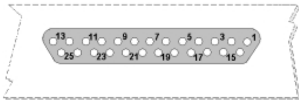
Fig. 3: DB-25 Connector Pinouts
